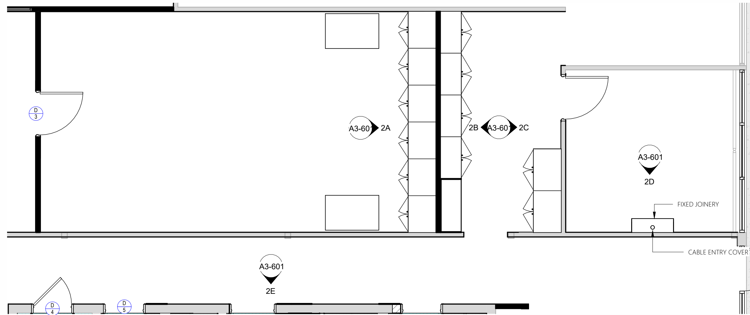
Internal Plan 2
