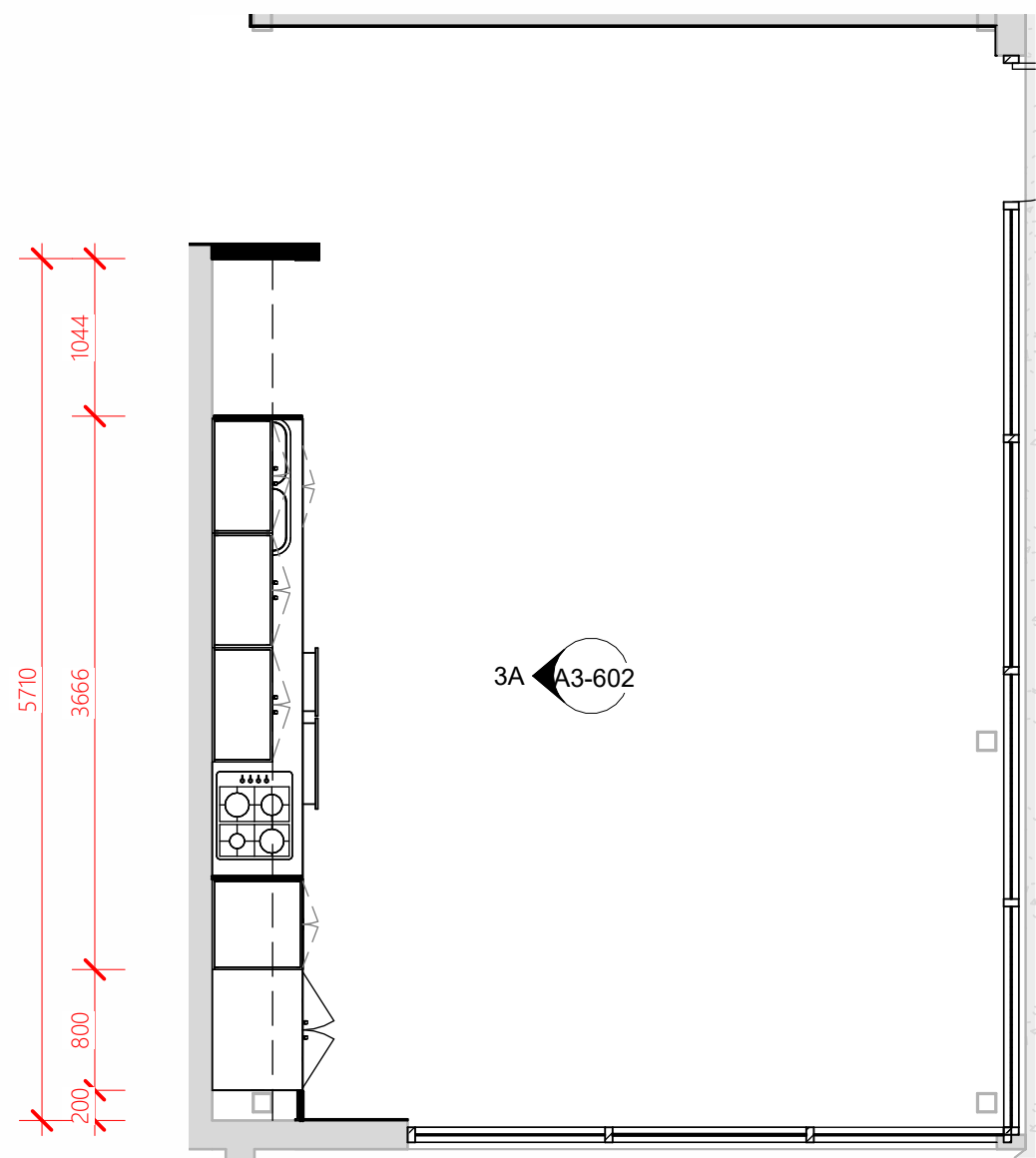
Internal Plan 3
