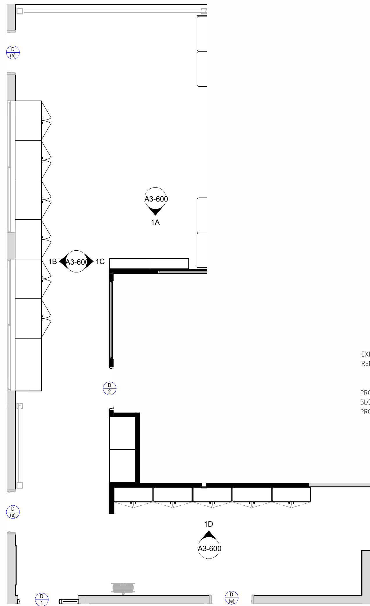
Internal Plan 1
