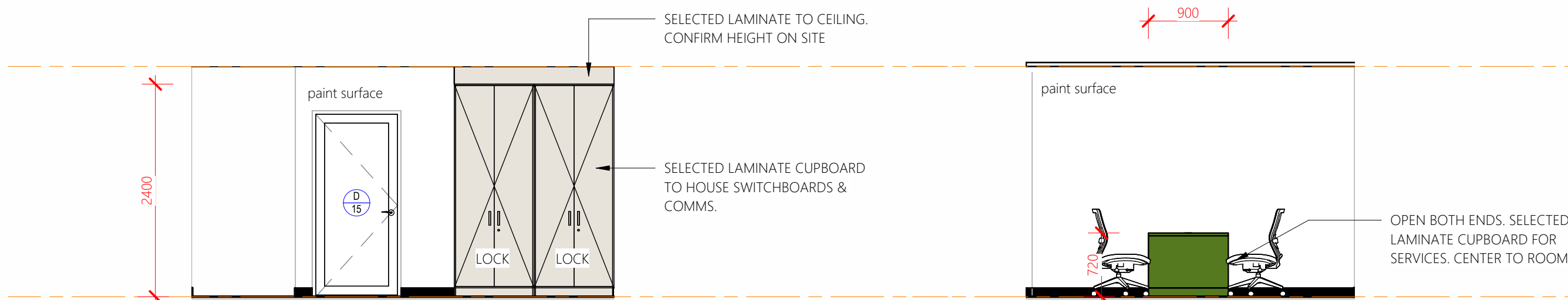
Elevation 2C
